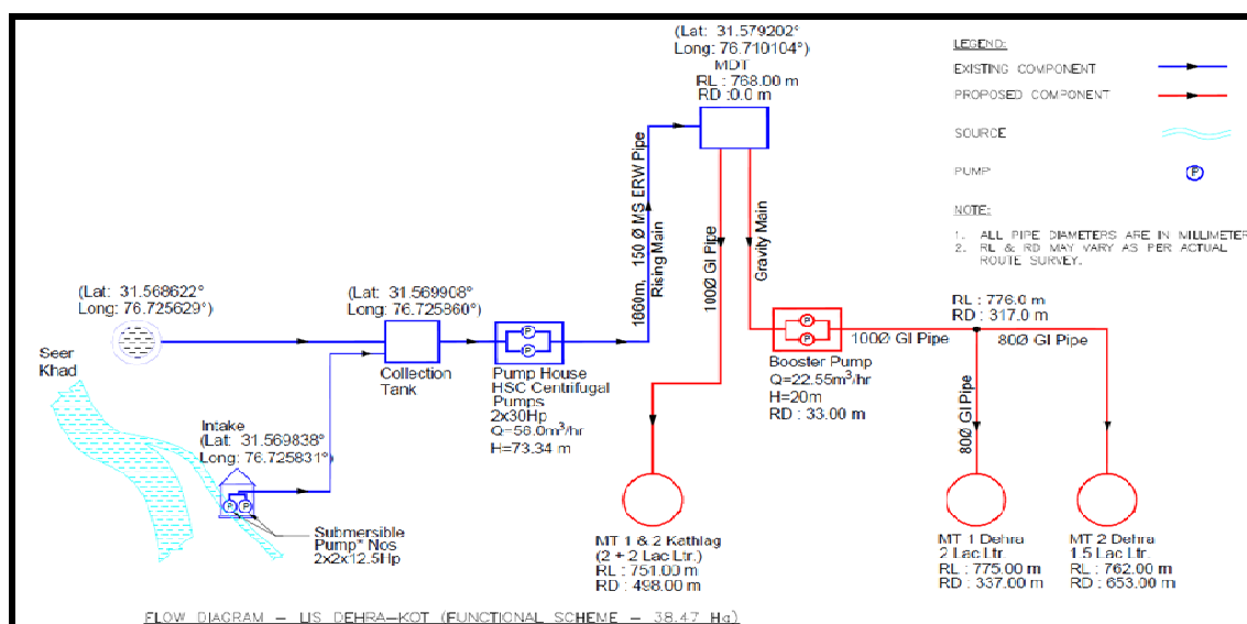
Flow diagram – Proposed LIS Dehra Kot
