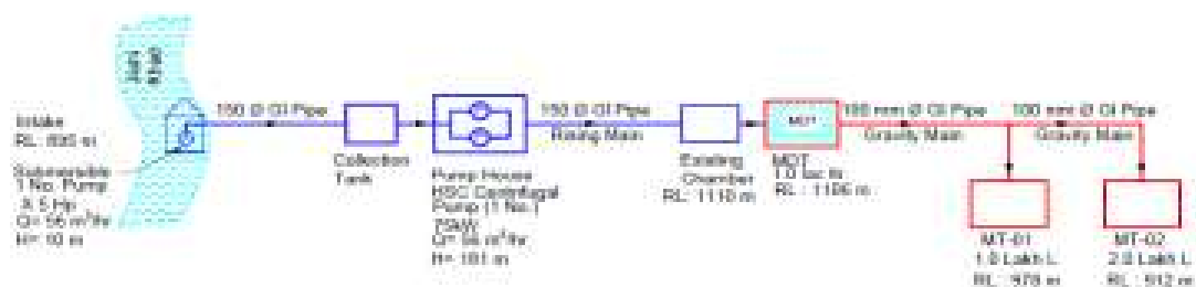
FLOW DIAGRAM - LIS SAWLA CLUSTER : CCA - 17.48 Ha (GOHAR BLOCK)
