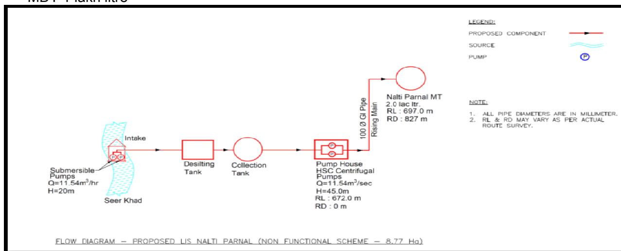
Flow diagram – Proposed LIS Nalti Parnal
