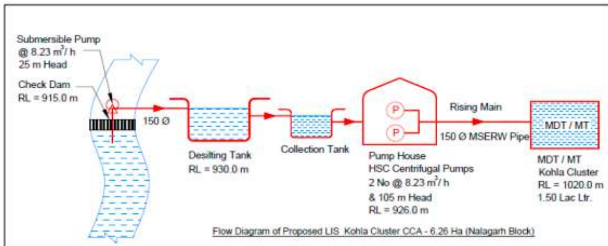
Figure 27: Flow Diagram of Proposed LIS Kohla
