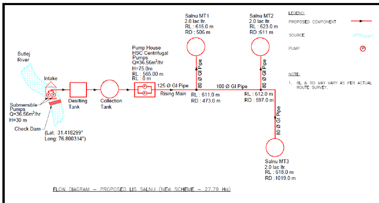
Flow diagram – Proposed LIS Salnu
