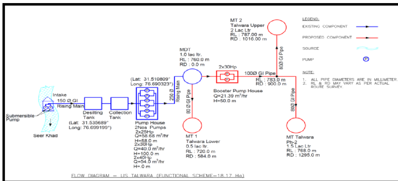
Flow diagram – Proposed LIS Talwara
