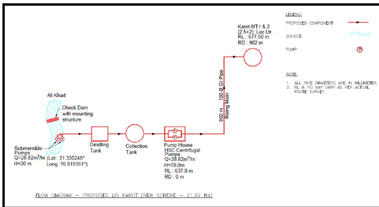
Flow diagram – Proposed LIS Karot
