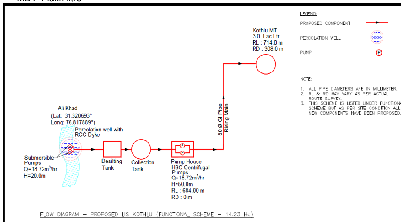
Flow diagram – Proposed LIS Kothlu
