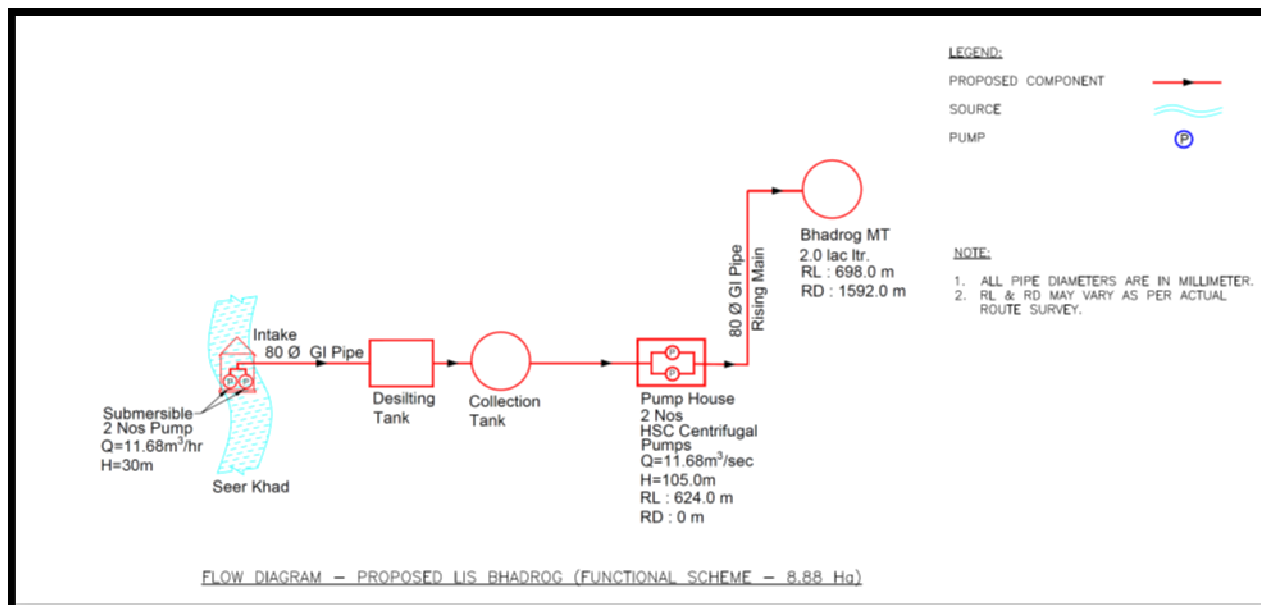
Flow diagram – Proposed LIS Bhadrog
