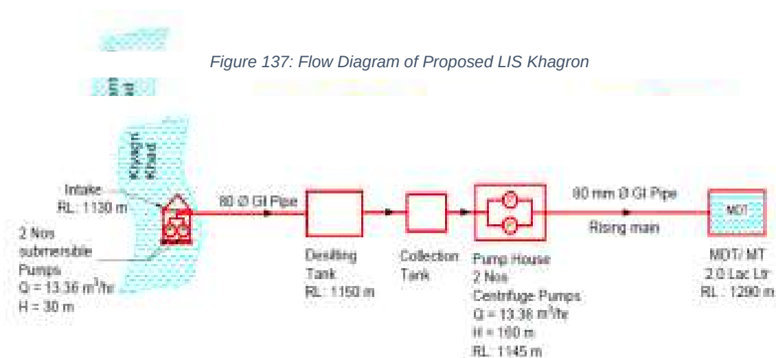
FLOW DIAGRAM - LIS KHARGAON CLUSTER : CCA - 10.15 Ha (SUNDERNAGAR BLOCK)
