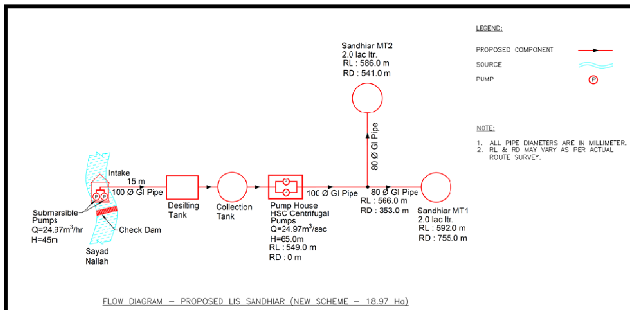
Flow diagram – Proposed LIS Sandhiar
