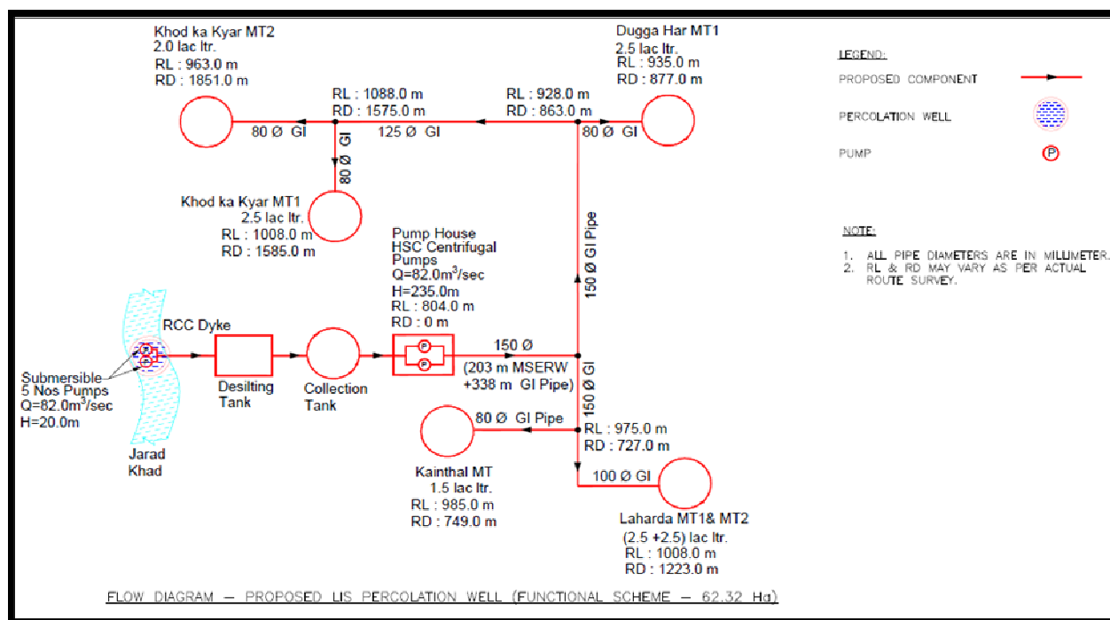
Flow diagram – Proposed LIS from Percolation well near Jarad Khad
