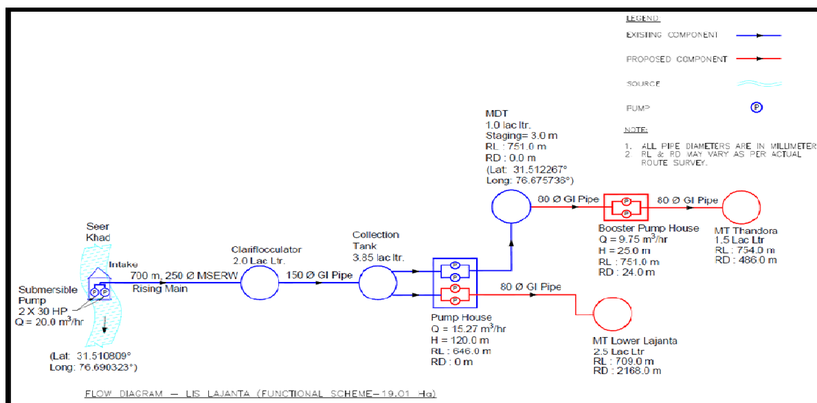
Flow diagram – Proposed LIS Lajanta
