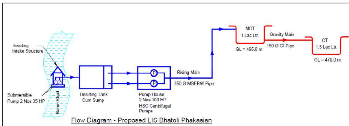
Figure 169: Flow Diagram LIS Bhatoli Phakasian
