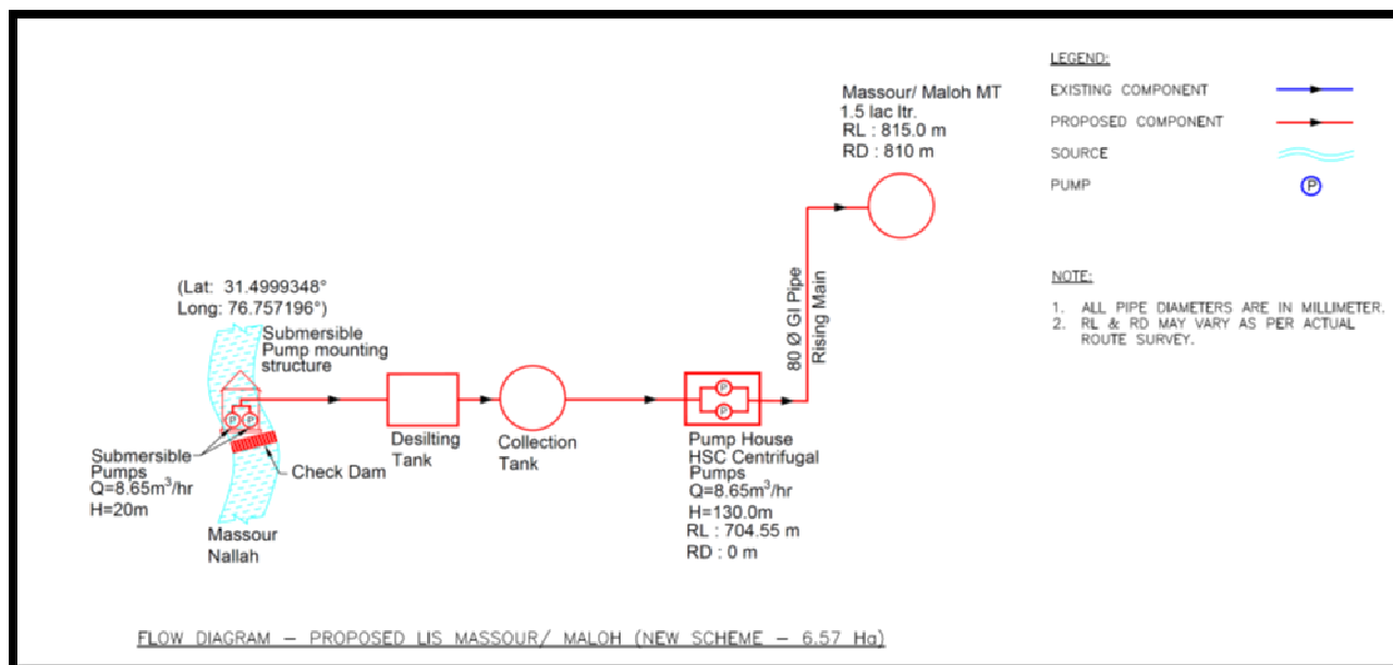
Flow diagram – Proposed LIS Massour/ Malloh
