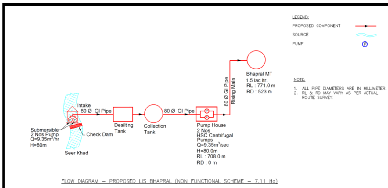
Flow diagram – Proposed LIS Bhapral
