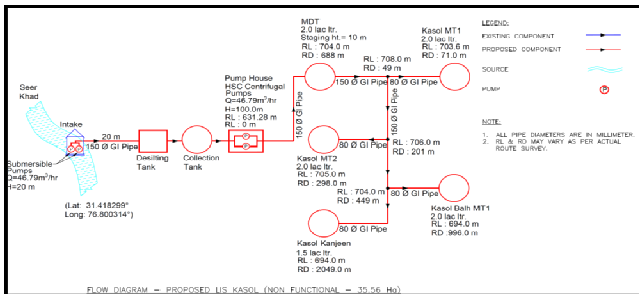
Flow diagram – Proposed LIS Kasol
