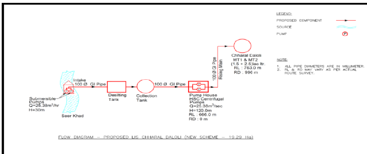
Flow diagram – Proposed LIS Chharal
