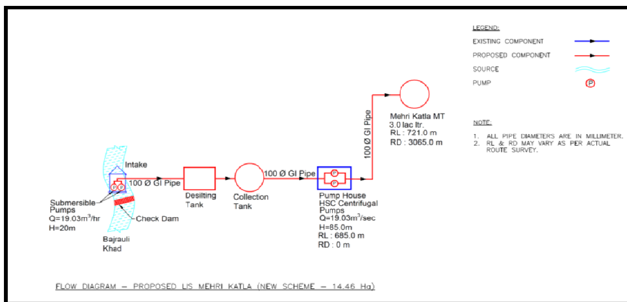
Flow diagram – Proposed LIS Meri Kathla
