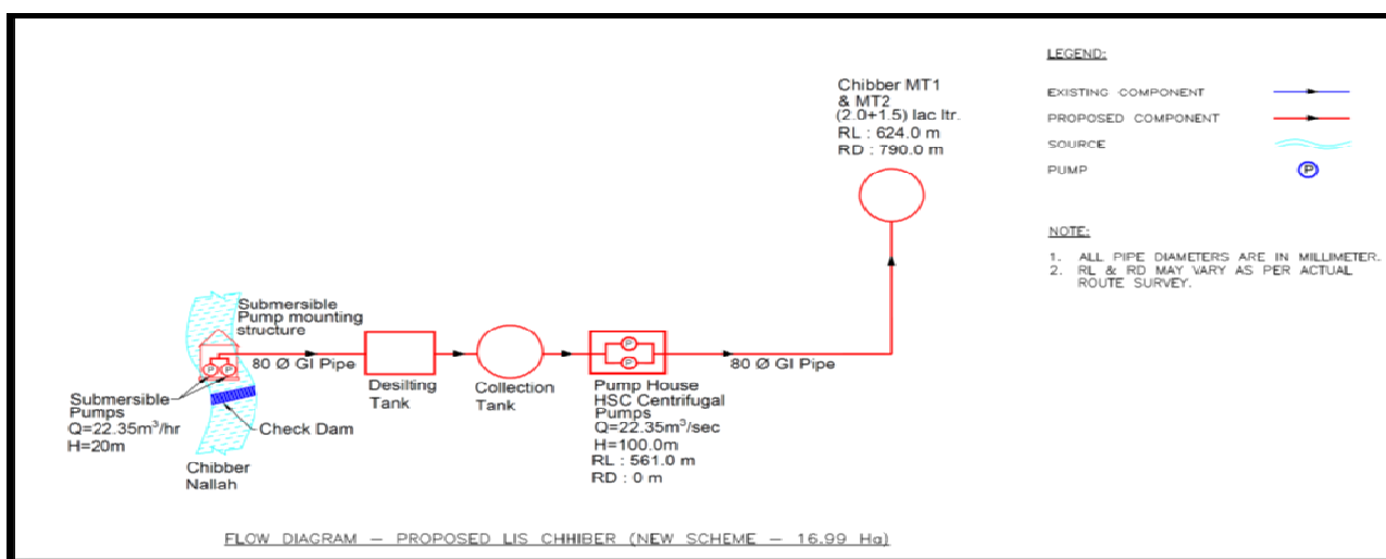
Flow diagram – Proposed LIS Chhiber
