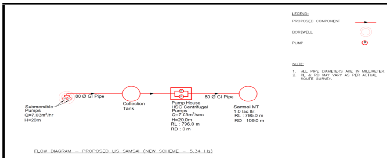
Flow diagram – Proposed LIS Samsai
