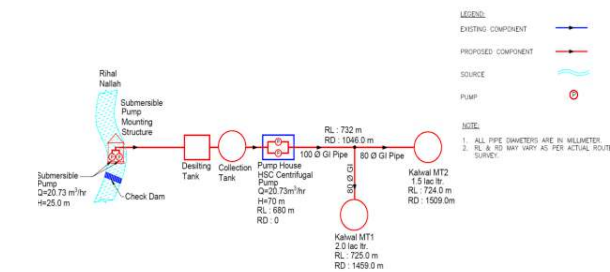
Figure 53: Flow Diagram of Proposed LIS Kalwal
